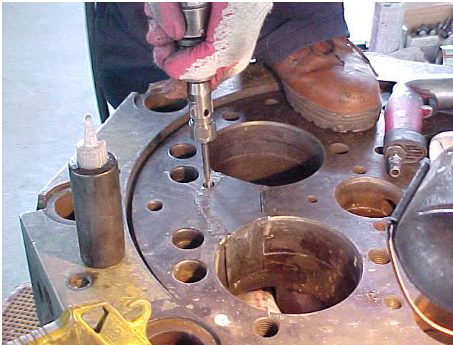
Stitching of Patch
