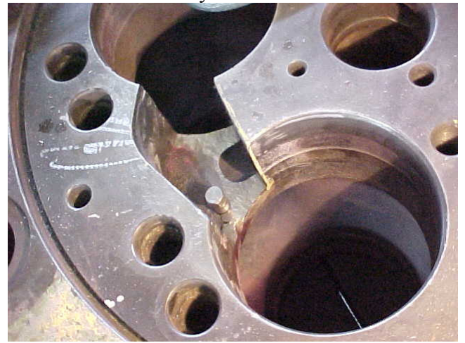
Stitching Repairs in Progress
