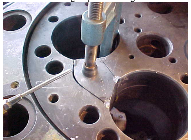
Installation of Patch
