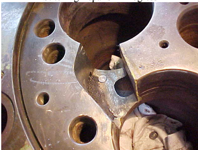
Stitching Repairs in Progress
