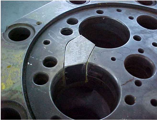
Fitting of Patch
